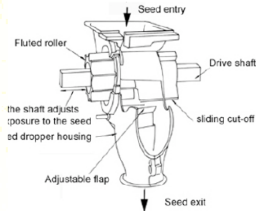
Fluted feed type seed metering mechanism
