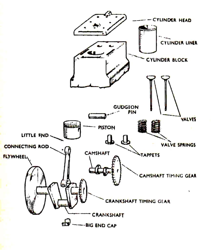
Engine components
