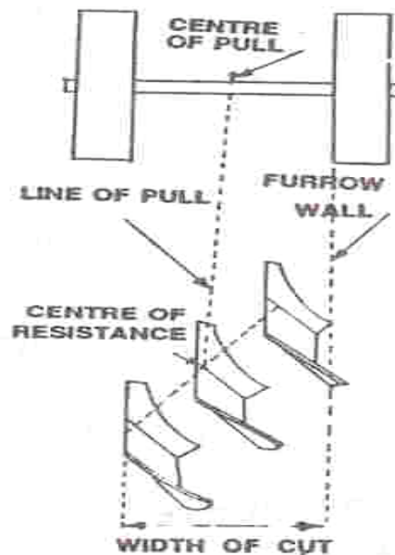
Centre of resistance
