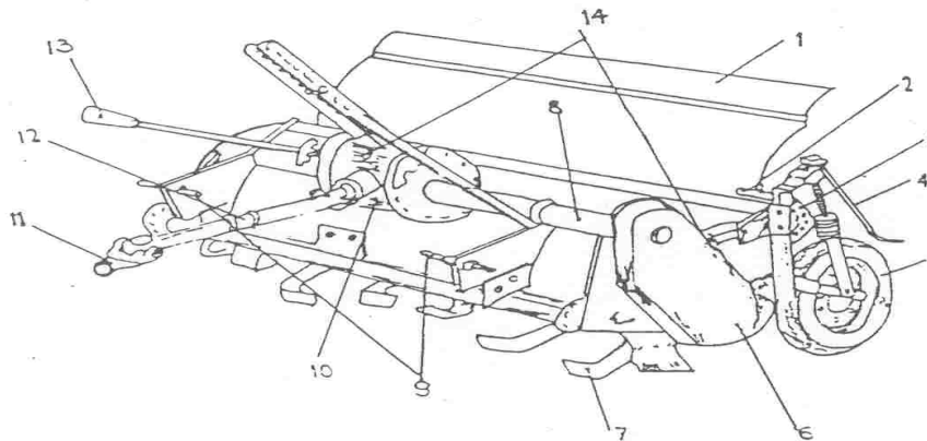
Fig.1. TRACTOR OPERATED ROTARY TILLER
