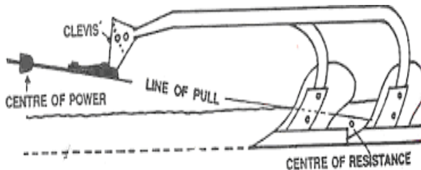
Clevis and line of pull
