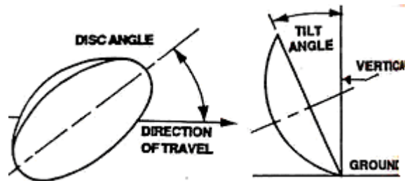
Angles of disc plough
