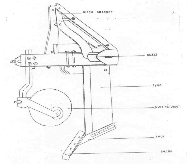
Sub soiler
