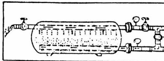
Sand Filter: Backwash Mode
