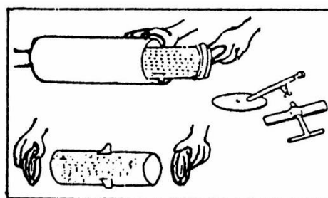
Cleaning of Screen Filter Rubber Caps
