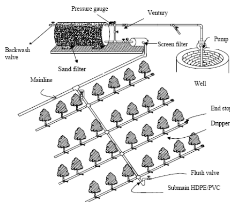
Fig. 1.1 Components of Microirrigation System
