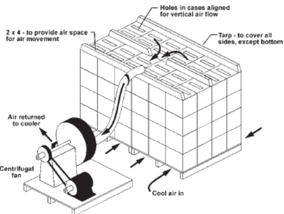
Fig.4. Forced vertical air flow
