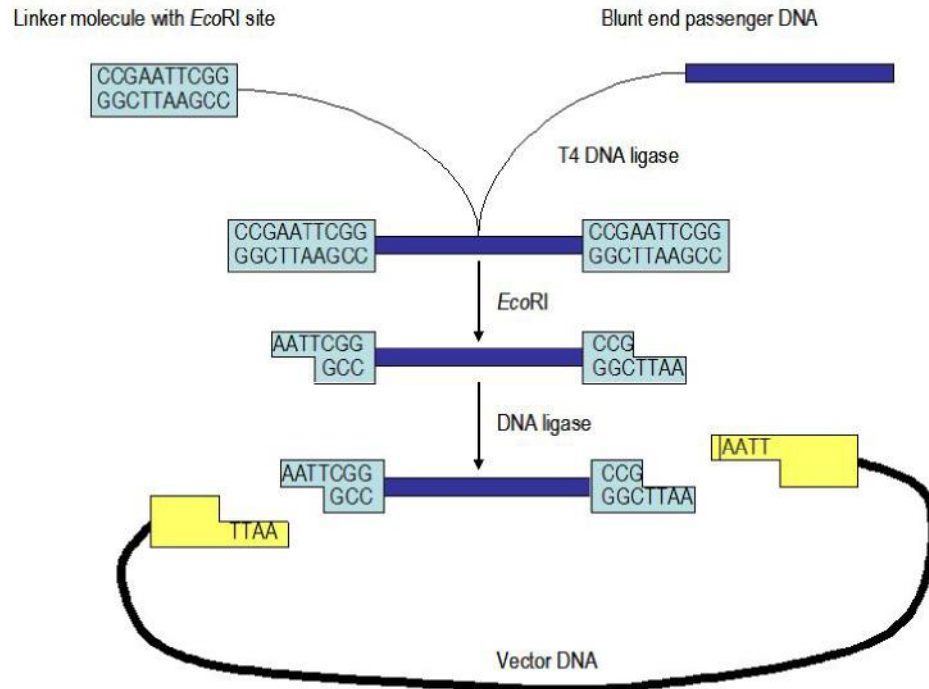
Joining of blunt end DNA to a vector using linkers
