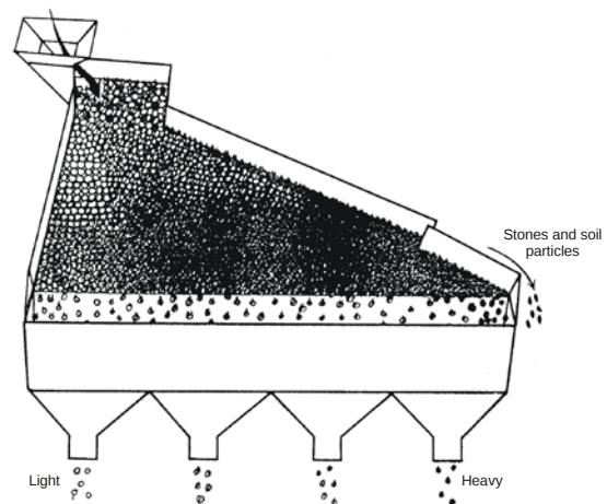
Working principle of the specific gravity separator
