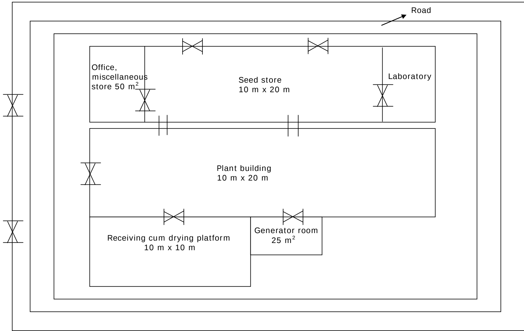
Building layout plan
